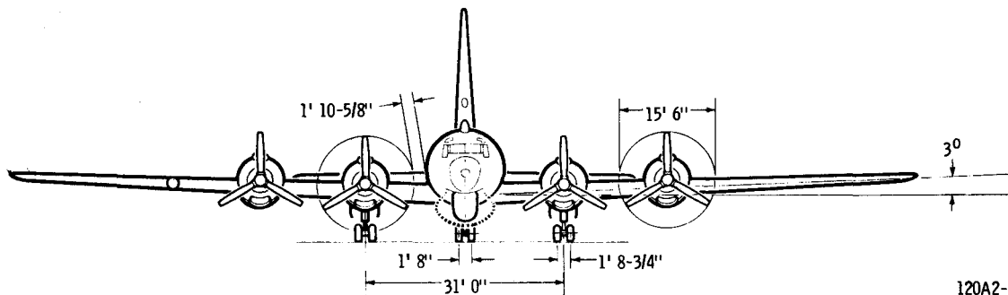
Aircraft Dimensions - Schematic
